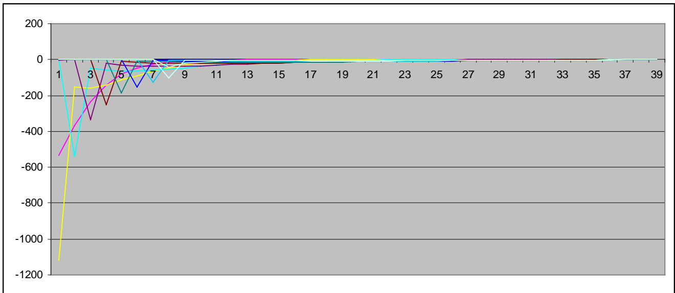
2 nd Gradient derivative (5B years,11x steps); Y =7000R; X =40x layers
