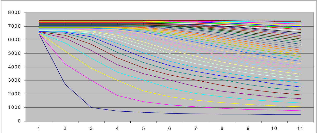
Chilling rate (layers); Y =7000R; X = 5B years (11x steps)
