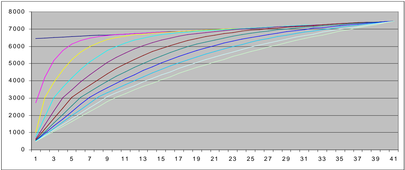
Crust gradient spread (5B years, 11x steps); Y =7000R; X =40x layers
